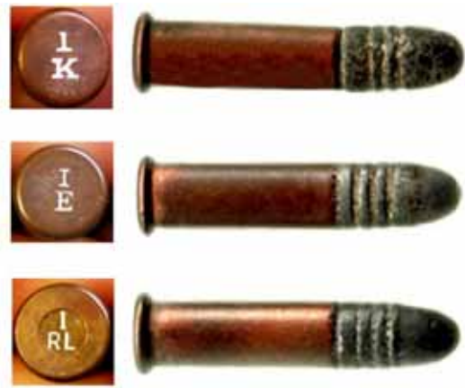
The three variants of the military Mk.1. Rimfire. Kynoch - Eley - and R.L. (Royal Laboratories) Woolwich Arsenal.
